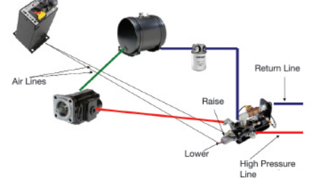
Combination Moving Floor/Dump Trailer System
