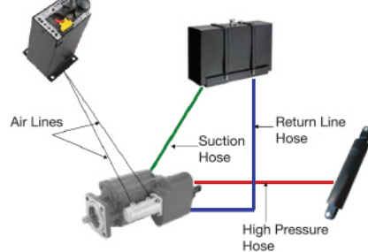
Dump Trailer Three Line System
