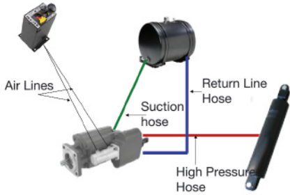
Dump Truck Three Line System
