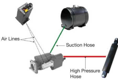
Dump Truck Three Line System
