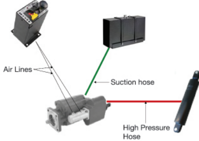
Dump Trailer Two Line System
